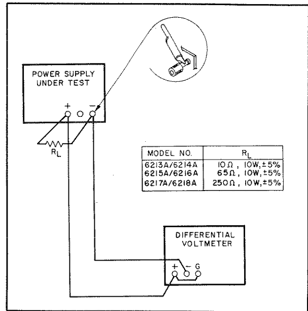
Figure 5-3. CV Load Regulation, Test Setup
